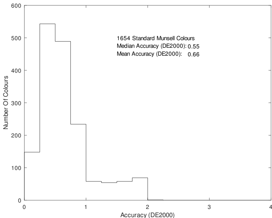
Figure 1: Histogram of Accuracies of Algorithm Output
